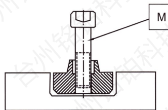
Extraction screw
