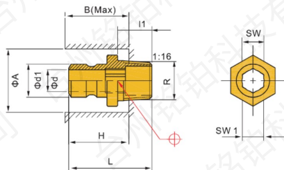
Connector plug with inner hexagon
