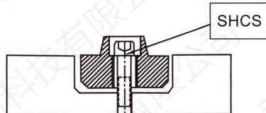
Fixation screw
