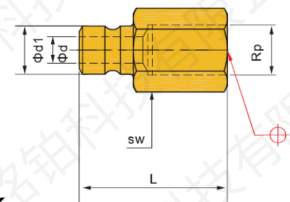
Connector plugs FSK and FSVK
